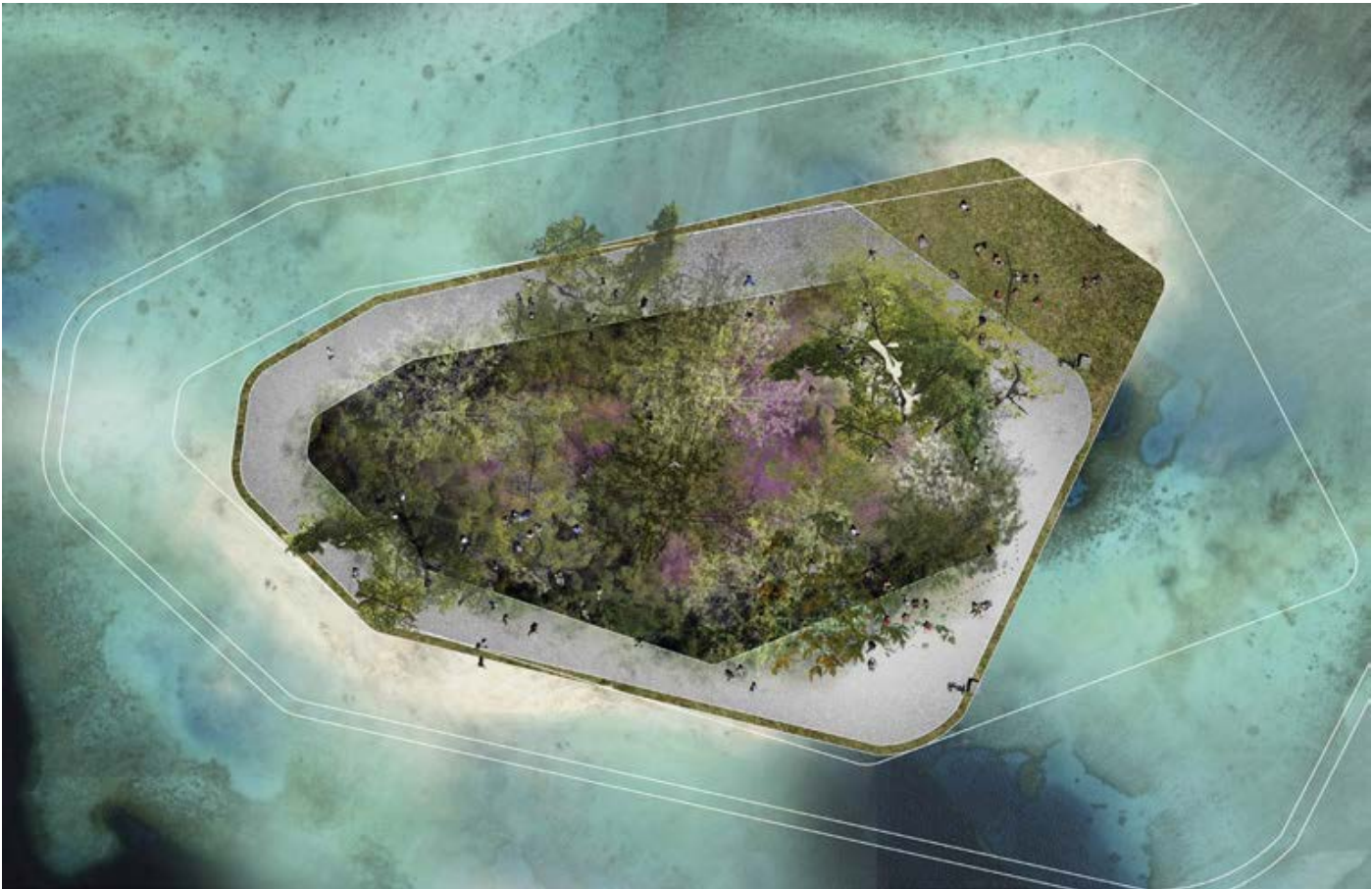
1) Fluvial Meander 2) Island
